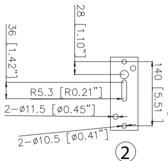
2 SILICON GASKET
