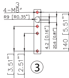
3 METAL PLATE
