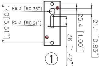
1 ROUND POLE PLATE
