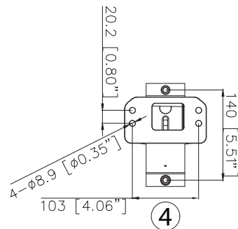
4 FRONT VIEW
